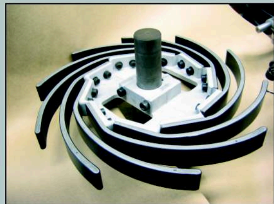
Schaufelrad Paddle wheel
